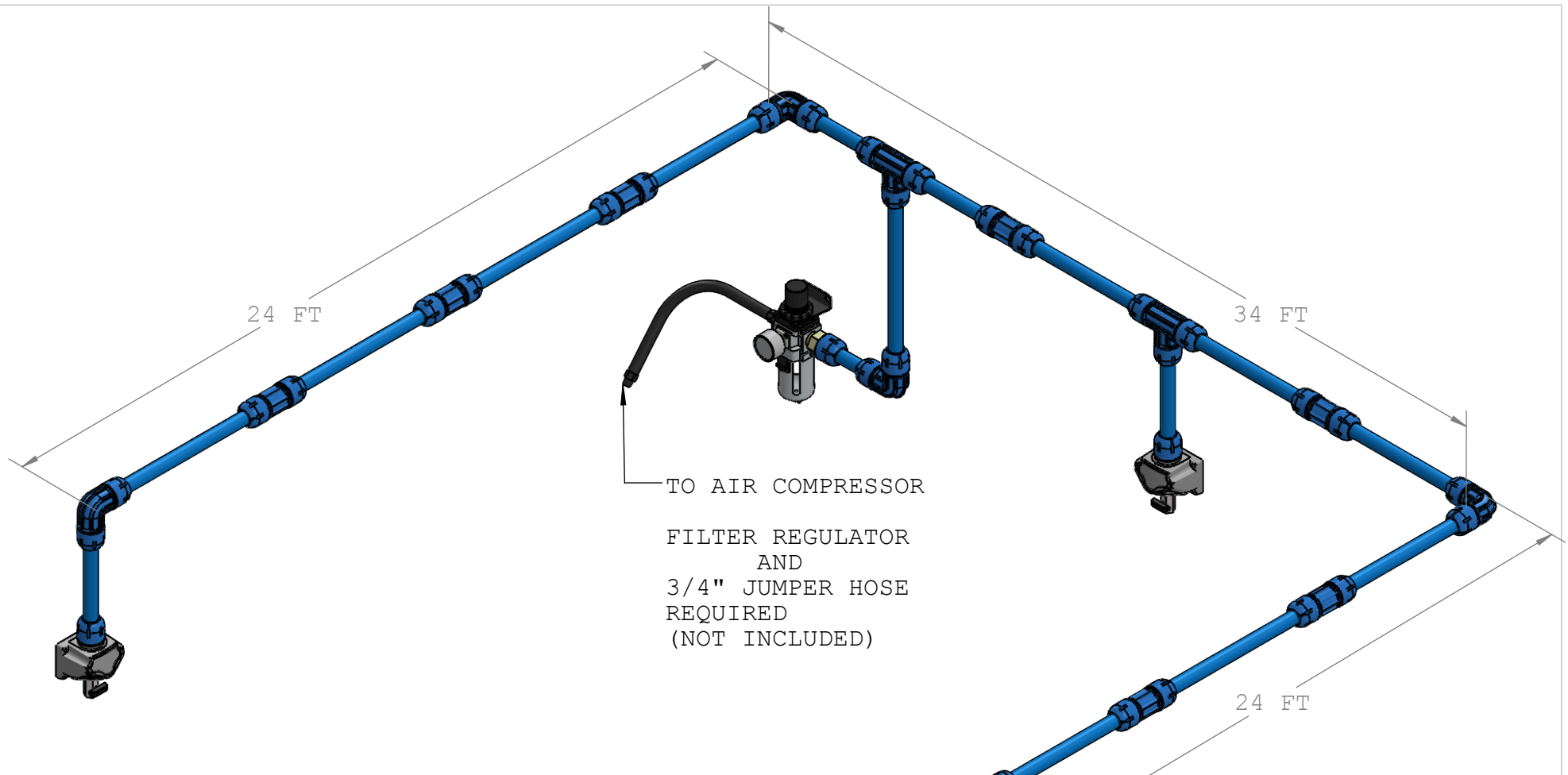
3/4 FASTPIPE KIT # F28070
