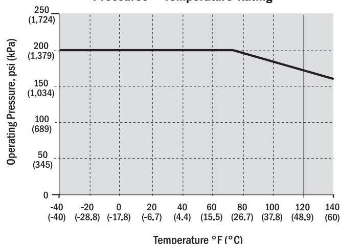
Figure 1 – Duratec Air-Line (3/8" to 1") Pressures – Temperature Rating
