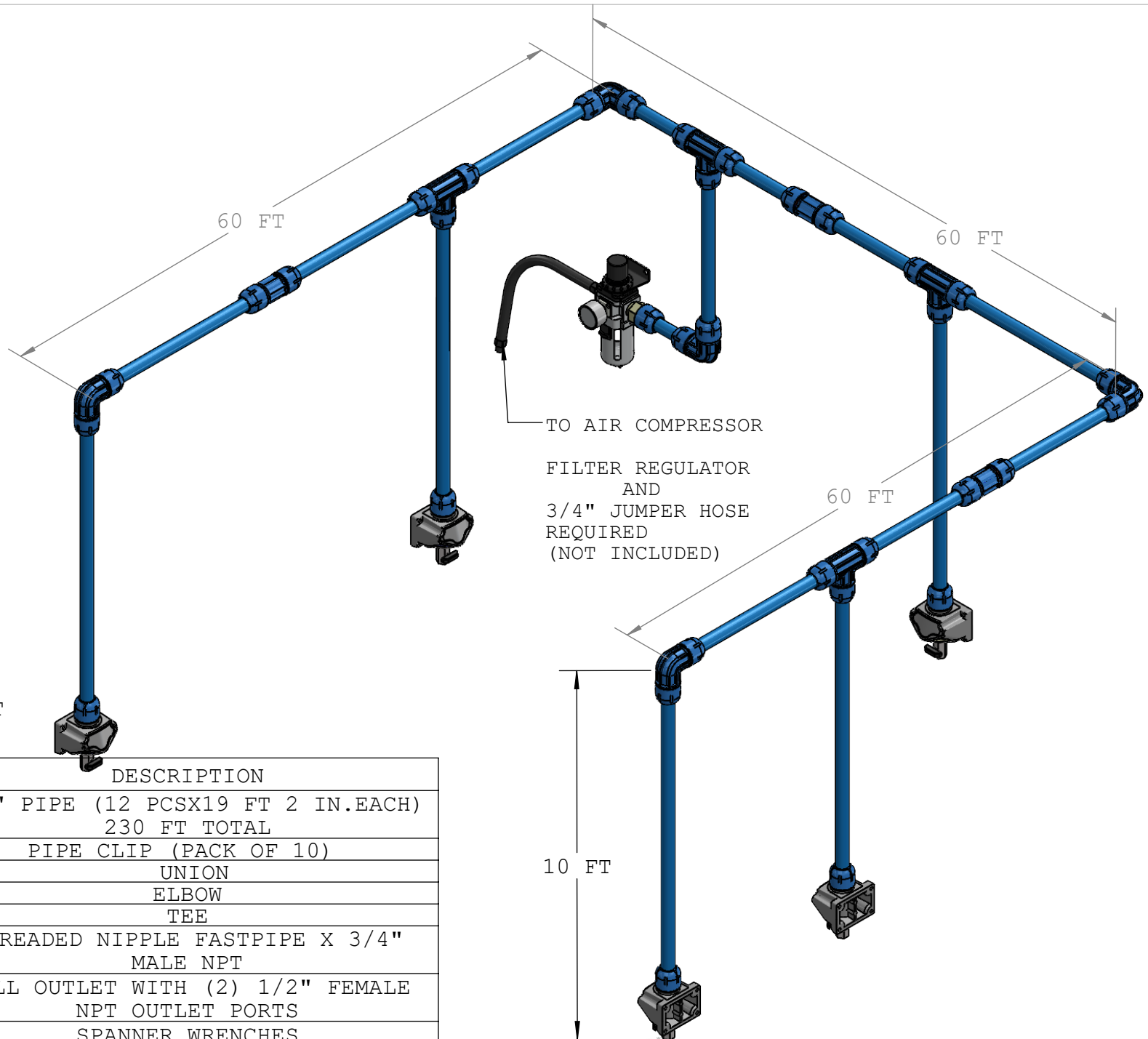
3/4" FASTPIPE KIT #F28099 Rev 1
